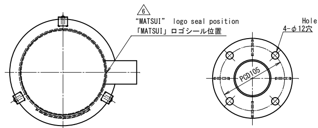
Figure from direction of A A矢視
