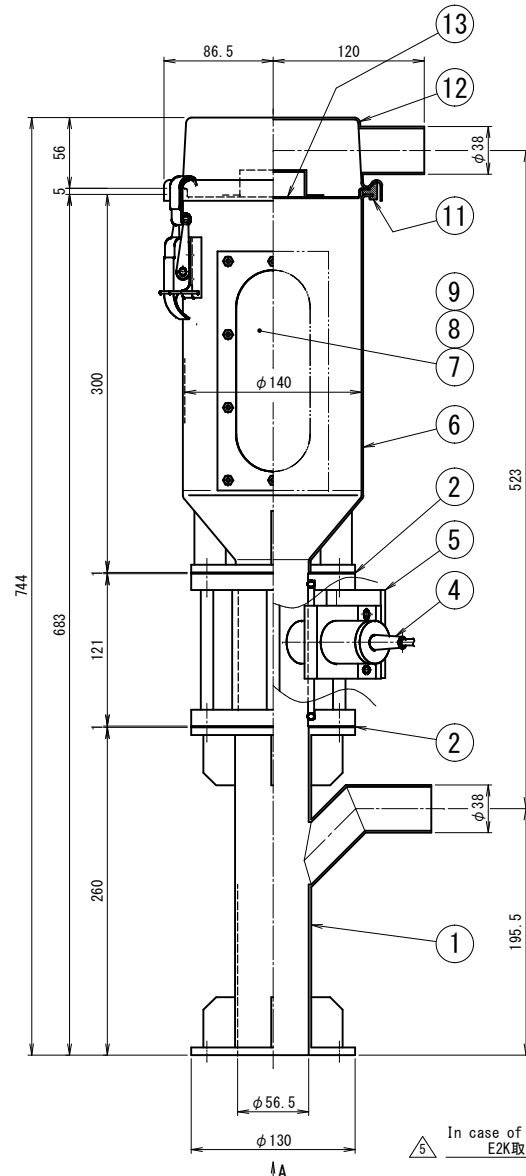
Figure from direction of A A矢視
